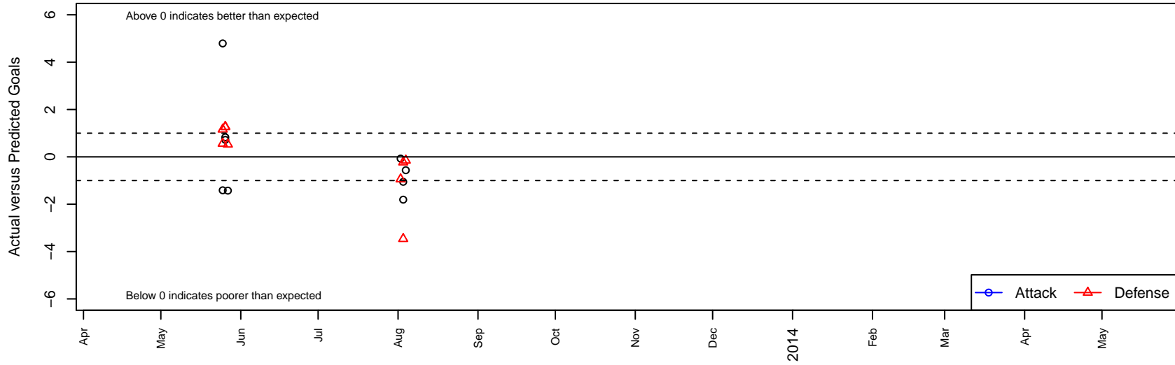
Redding Kaos Hurricanes B01 Dots are actual minus expected GF (blue circles) and GA (red triangles). Blue line is smoothed change in attack strength. Red is smoothed change in defense strength.
